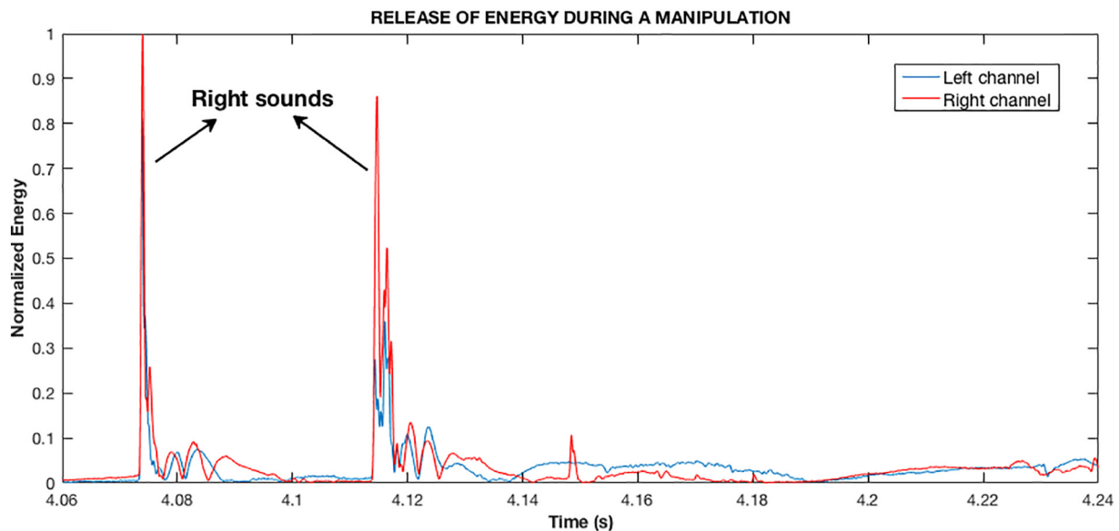
Fig 4. Amount of energy released over time for the right and left accelerometry channels.
