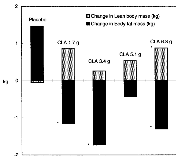
FIGURE 2 Body fat mass and lean body mass in obese and overweight men and women given placebo or varying amounts of CLA. Body fat mass and lean body mass were measured by dual-energy X-ray absorptiometry at wk 0 and 12 and expressed as the difference between the values at wk 0 and 12. * P \leq 0.05 for significance of difference between CLA treatment group and placebo group.
