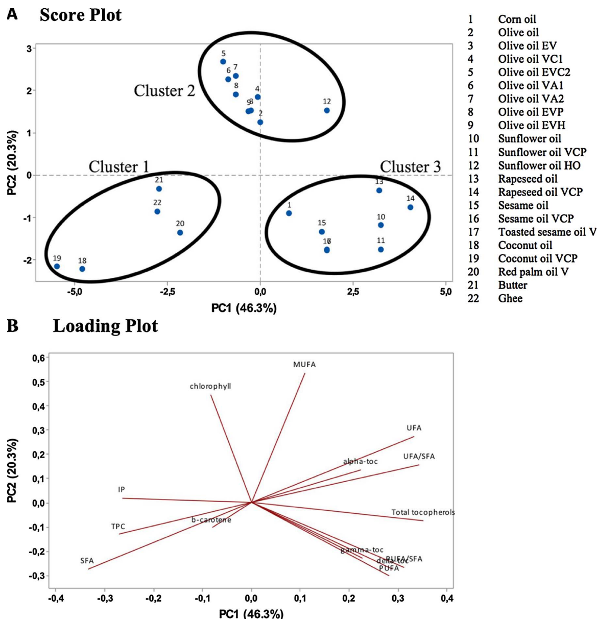
Fig. 2. Score plot (A) and loading plot (B) for oil and fat samples ( n = 22 ). Matrix analysis included the following variables: IP, \alpha -tocopherol (alpha-toc), \gamma -tocopherol (gamma-toc), \delta -tocopherol (delta-toc), total tocopherols, \beta -carotene (b-carotene), chlorophyll, TPC, SFA, MUFA, PUFA, UFA, and PUFA/SFA and UFA/SFA ratios.
